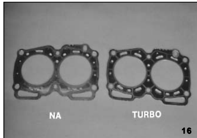
Head Gaskets
