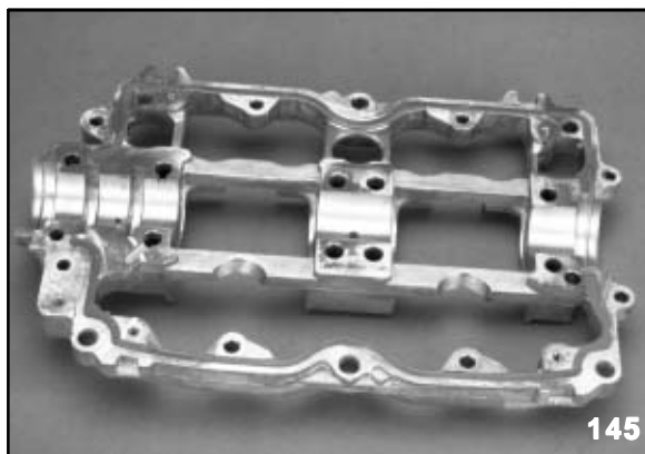
Camcase Sealing Points
