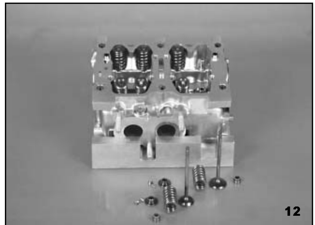
Valve Components
