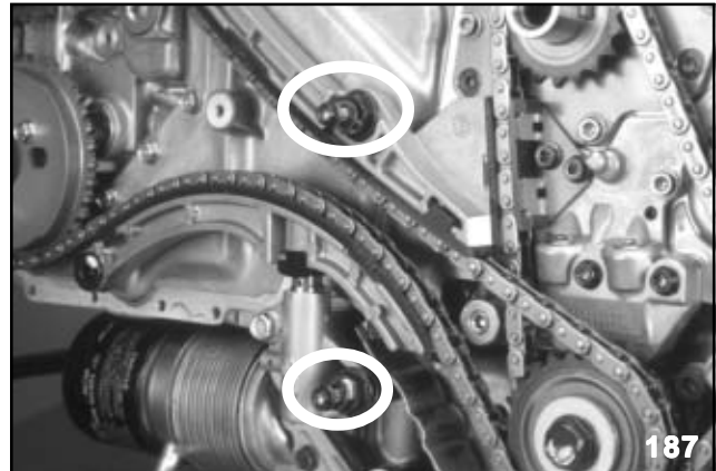
Outer Cover Bolts
