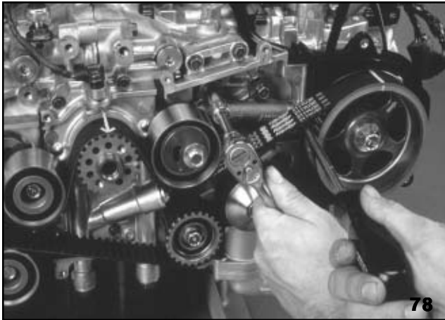
Loading Tensioner
