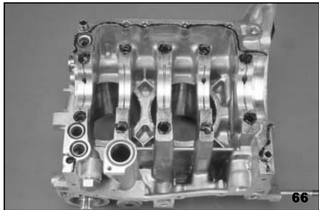
Crankcase Sealer and O-Rings
